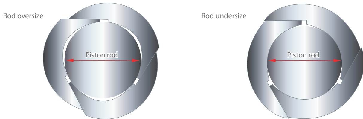
Fig.6 | How a standard bore packing ring will fit an oversize and an undersize rod. Note: joints remain in contact
