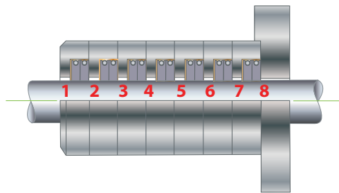
Fig.10 | Pressure drop pattern through a packing
