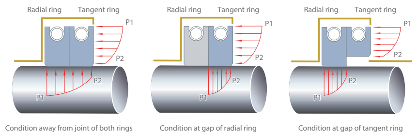
Fig.9 | Pressure drop across a pair of packing rings
